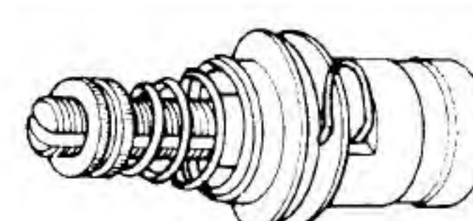
97800 TENSION UNIT
