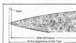
Test of Wear with a PD Needle
