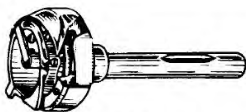
240207, 240197 (HEAVY SHAFT W/SLOT) HOOK & BOBBIN CASE F/111W100, 101, 102, 103, 153, 154
